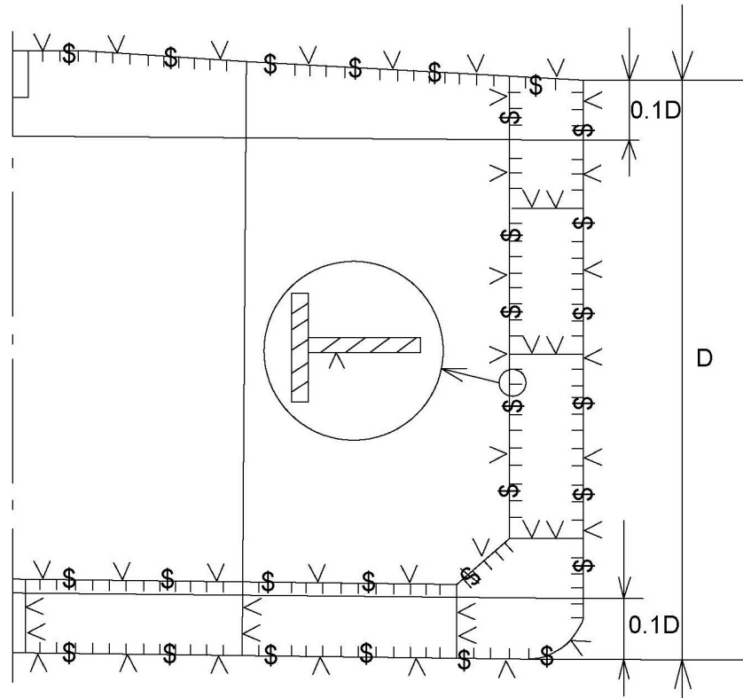
Figure 5 - Transverse section
